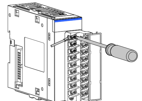
Figure 5 Connecting cable to terminal block
