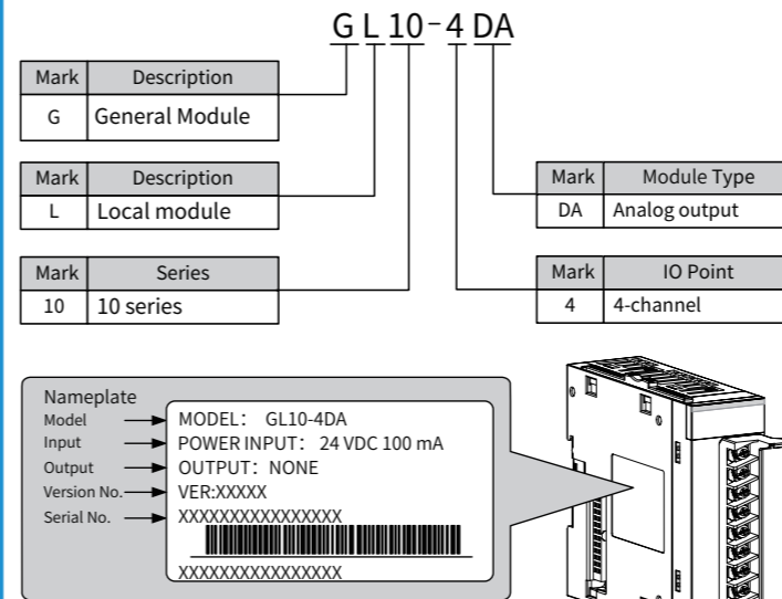
Figure 1 Description of model and nameplate
