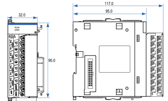
Figure 3 Mounting dimensions diagram (in mm)
