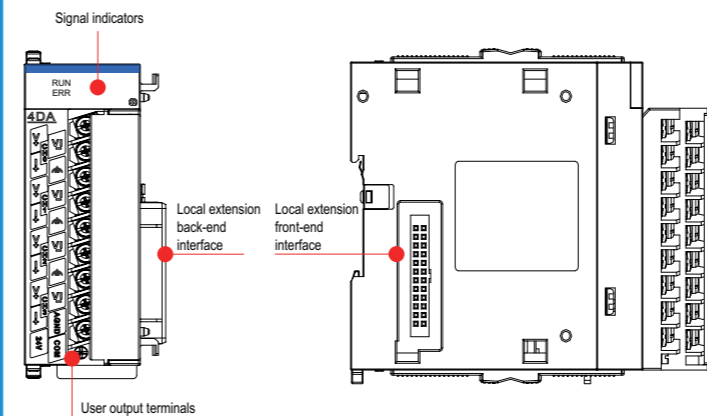
Figure 2 Diagram of the analog output modules interface
