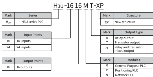
Figure 1-2 Designation rule of H 3U -1616MT/R-XP, H 3U -2416MR/T-XP
