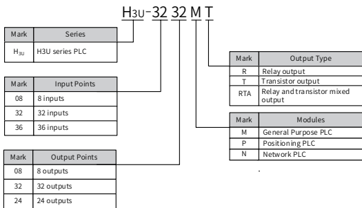
Figure 1-1 Designation rule of H 3U -0808PMRTA (selling stopped) , H 3U -3232MR/T, H 3U -3624MR/T
