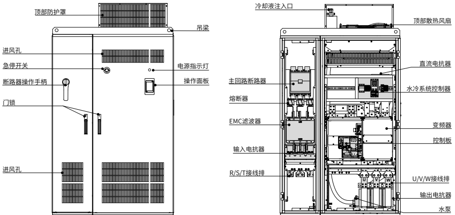
图 1-4 MD290T500G-A~MD290T630G-A、MD290T560P-A~MD290T800P-A（带辅助配电机柜）各部件说明
