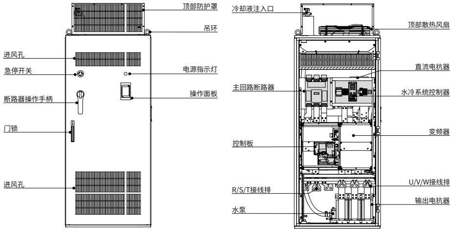
图 1-3 MD290T500G~MD290T630G、MD290T560P~MD290T800P（标准机柜）各部件说明
