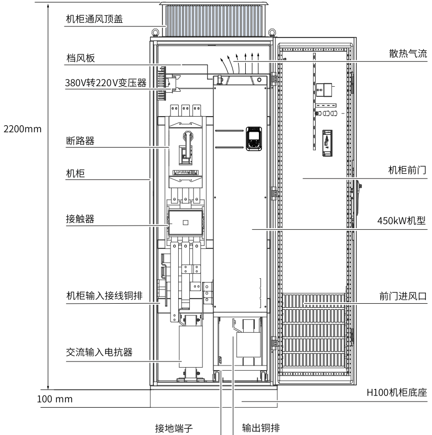
图5-4 T12机型机柜布局推荐
