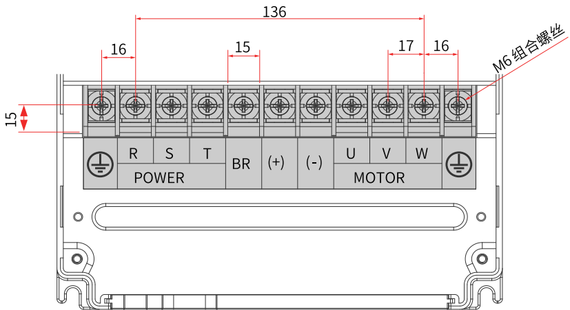
图8-12 T5机型主回路端子尺寸 (mm)
