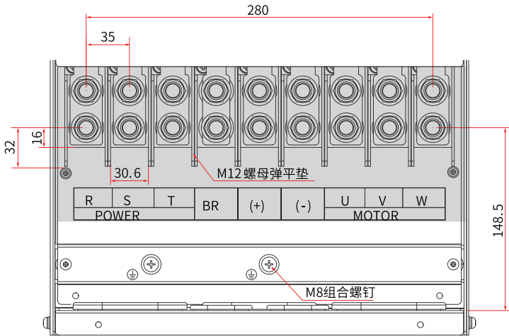
图8-15 T8机型主回路端子尺寸 (mm)
