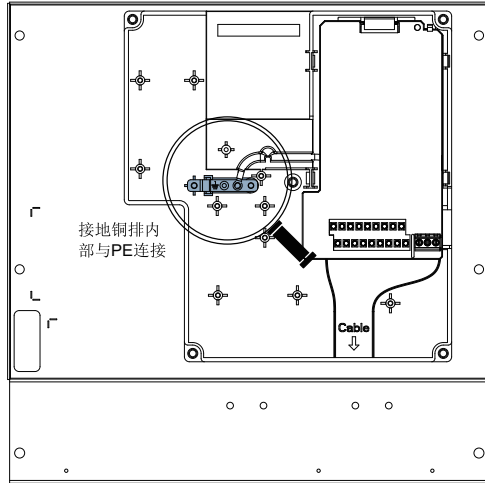
图8-53 PG卡安装螺钉
