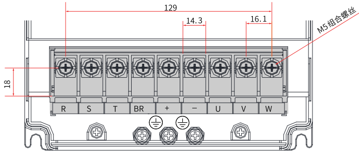
图8-11 T4机型主回路端子尺寸 (mm)
